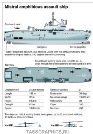
Mistral amphibious assault ship
